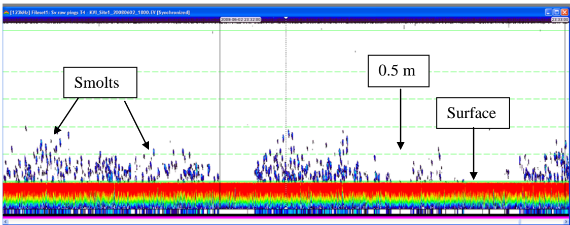
Figure 21. Echogram of smolt detected 2 May, 2008 at Site 1. Dashed green lines signify 0.5 m depth strata and show majority of smolts are in the upper 1.0 m. (EchoView® 4.5 software displays echogram of smolt data as “upside down” due to up-looking transducers.)
