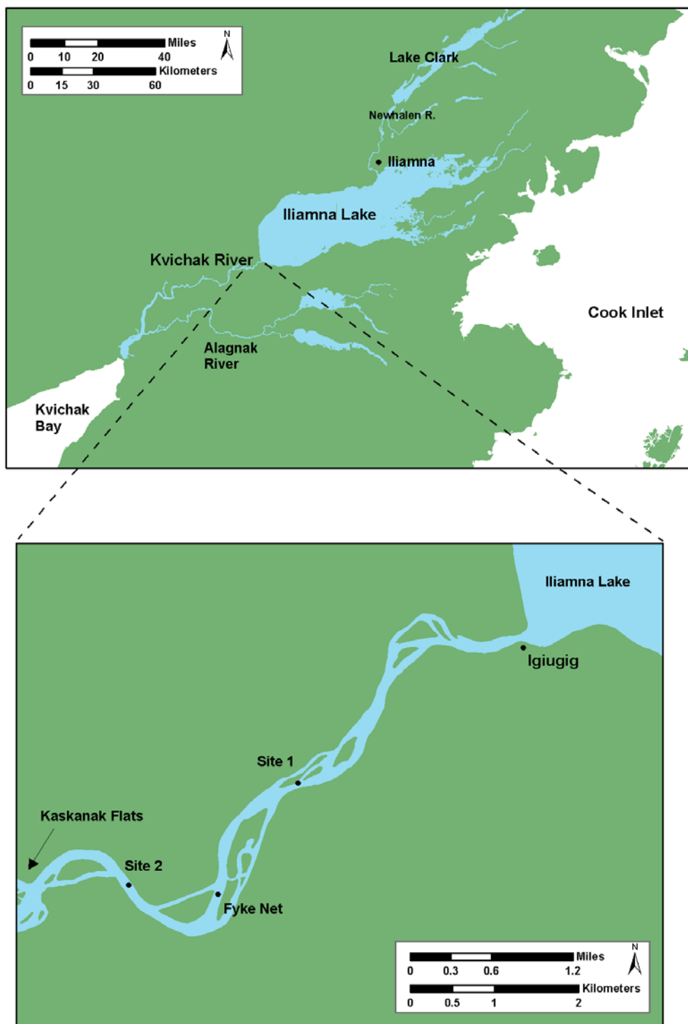
Figure 3. Map of study site on the Kvichak River showing locations of sonar sites 1 and 2, plus the fyke net location used for smolt sampling, 2008.
