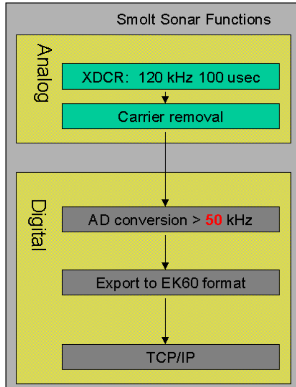
Figure A-1. Functional overview of a sonar pod used on the Kvichak River in 2008.
