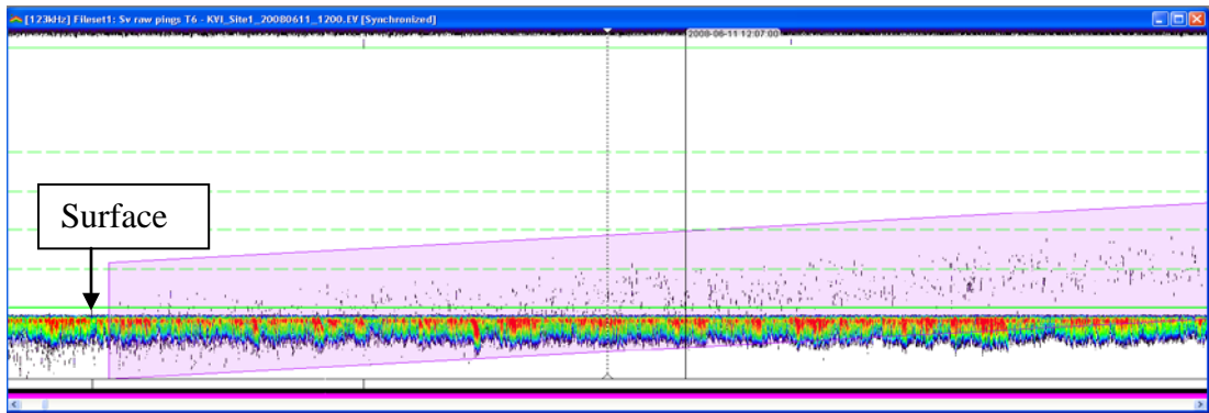
Figure 23. Echogram of cross-talk (shown in highlighted purple region) between transducer six and seven, 2008. (EchoView® 4.5 software displays echogram of smolt data as “upside down” due to up-looking transducers.)
