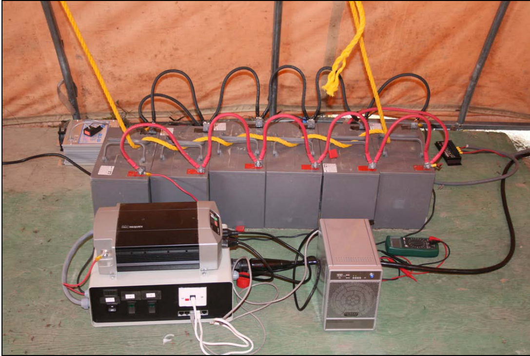
Photo 3. Control box, NAS and power source for the site 1 sonar system housed in Weather Port tent, 2008.
