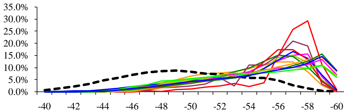
Figure 10. TS distribution of single targets from each transducer (dashed line is transducer 6 at site 1) for the first week of sampling, 2008.
