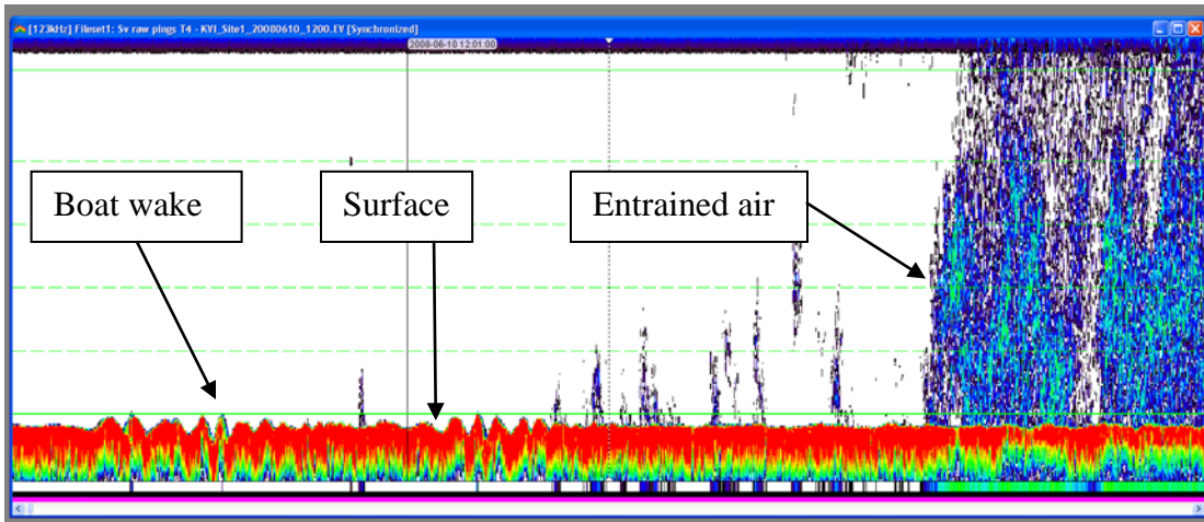
Figure 20. Echogram of noise generated by boat passage on 10 June, 2008 at Site 1, note the boat wake that precedes the noise created by entrained air from the propeller. (EchoView® 4.5 software displays echogram of smolt data as “upside down” due to up-looking transducers.)
