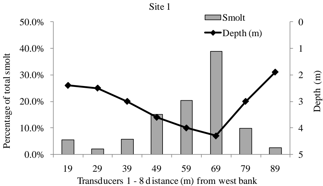
Figure 5. Site 1 bottom profile (based on transducer depth) plus cross river distribution of smolt detected, 2008.
