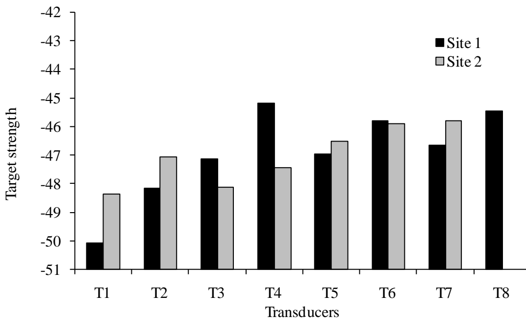
Figure 12. EMS deconvolution estimates of TS by transducer, 2008.
