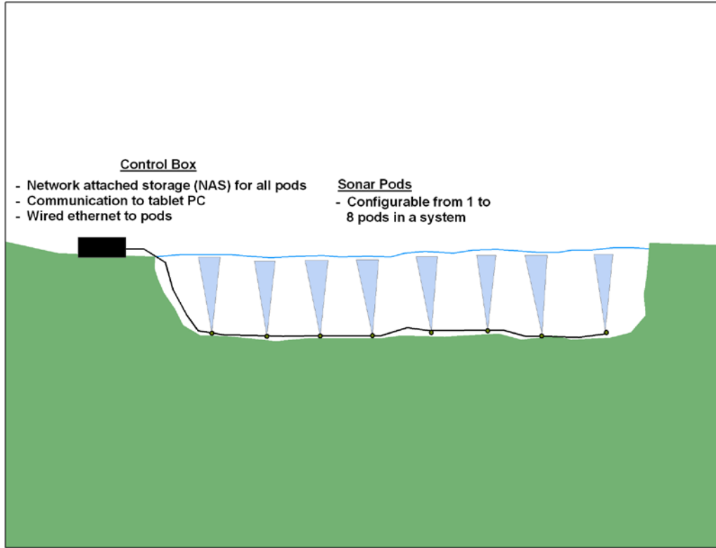
Figure 4. Conceptual drawing of smolt sonar designed for rivers in the Bristol Bay region, 2008.
